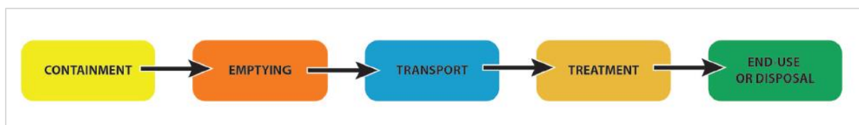
Figure 16: The Faecal Sludge Management Service Chain
